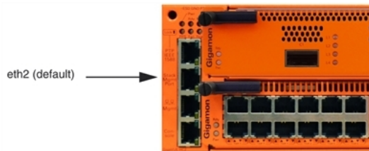
Figure 93 Stack Port Location on GigaVUE-HC2 Front
