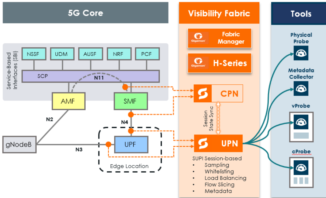
Figure 28 5G Stand Alone Packet Core Network
