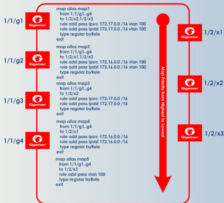
Figure 7 Sending Subnets and VLANs to Different Ports
