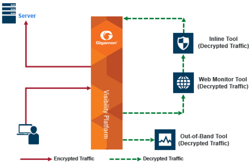
Figure 78 Inline SSL Decryption Example, Outbound
