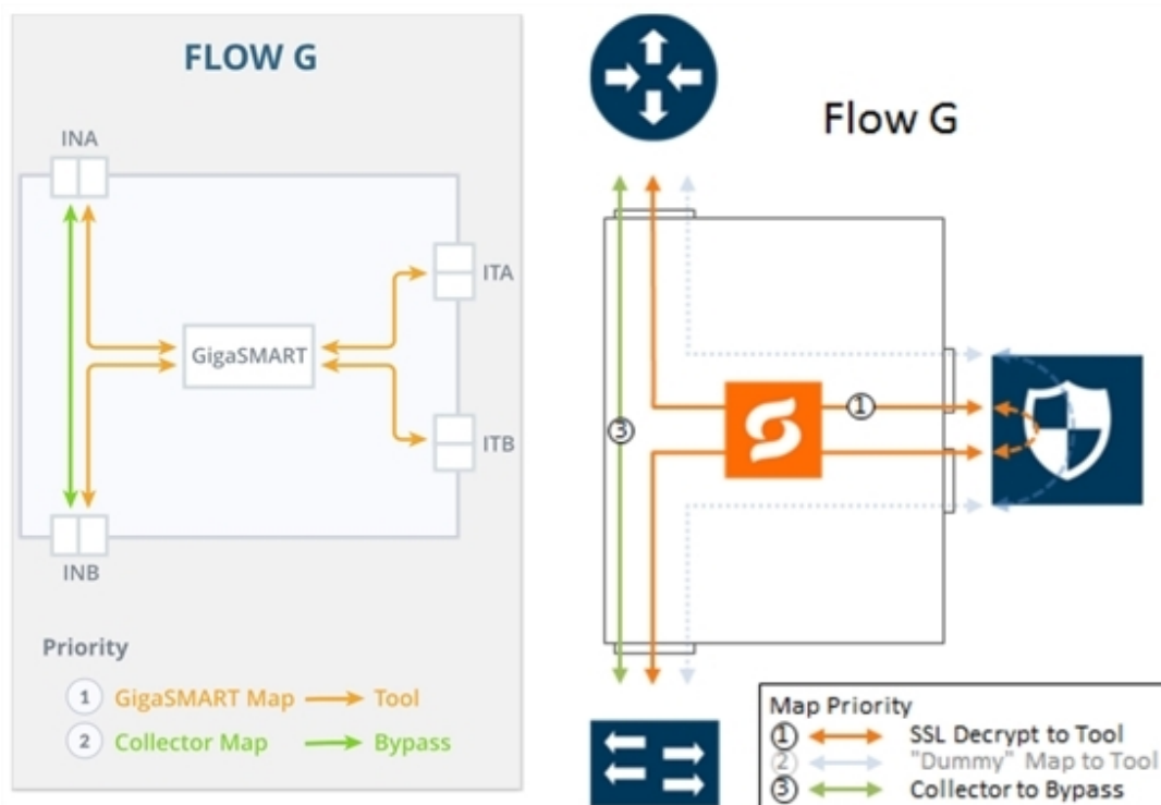
Figure 104 FLOW G Views
