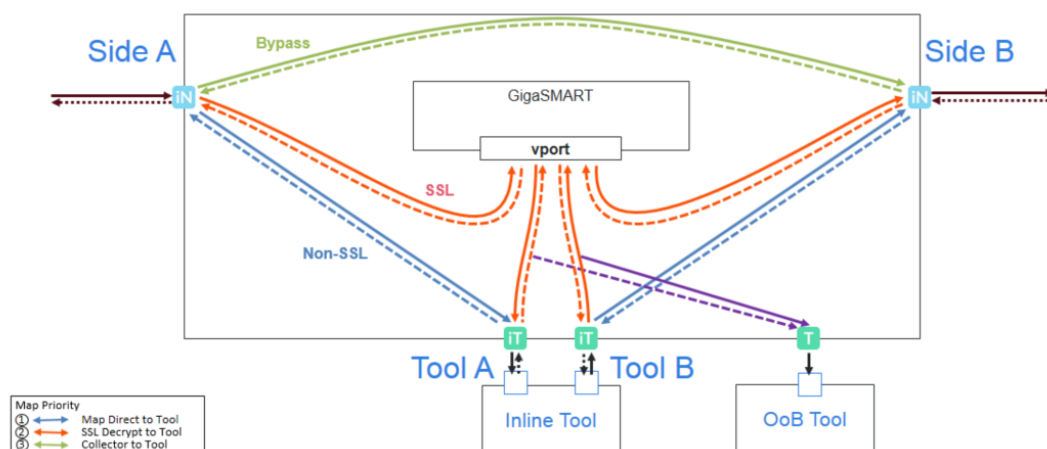
Figure 92 Packet Flow for Inline SSL Decryption
