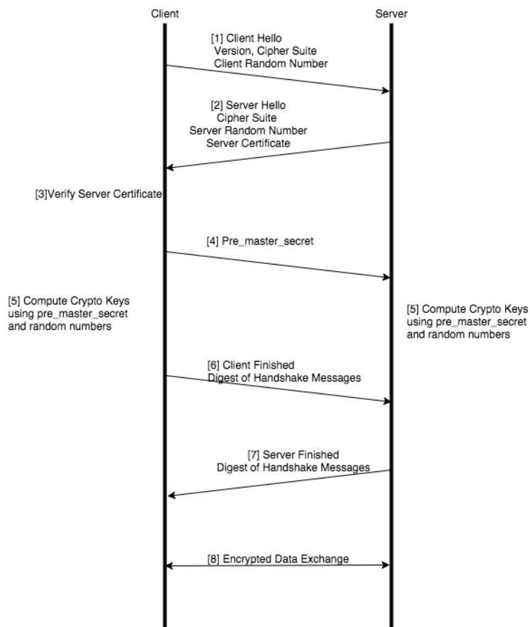
Figure 79 Basic RSA SSL Handshake
