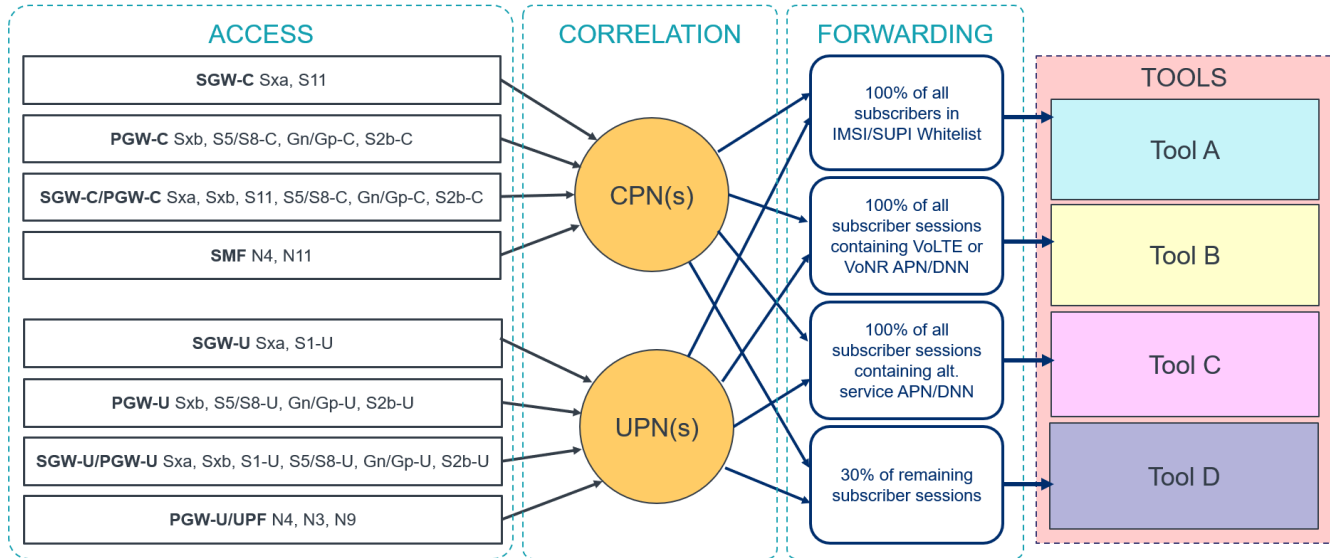
Figure 29 CUPS Traffic Visibility Solution
