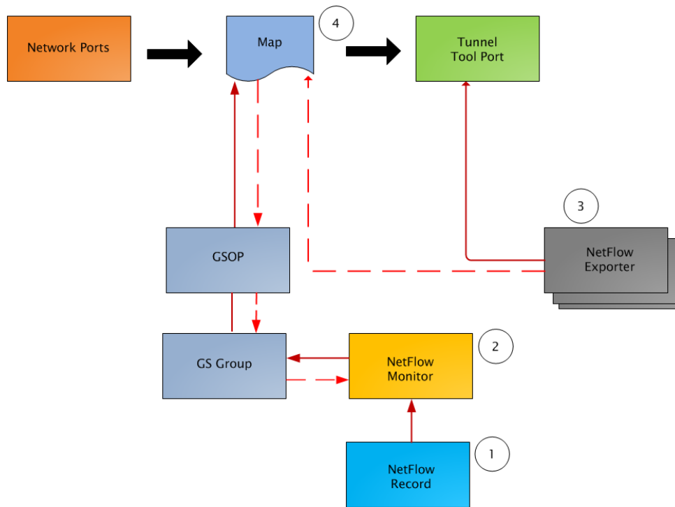
Figure 68 NetFlow Generation Components
