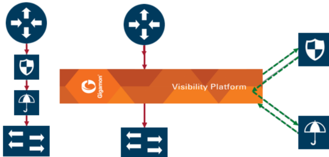
Figure 88 Serial Inline Tool Arrangement
