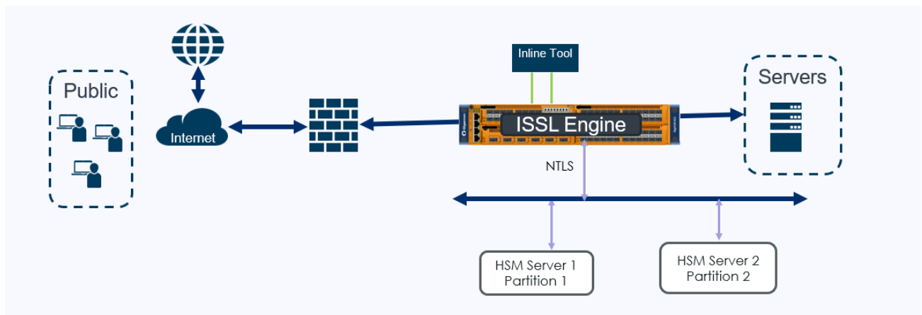
Figure 126 iSSL with Thales Luna - Inbound support
