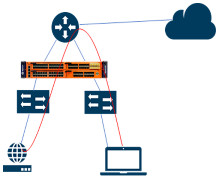
Figure 85 Inline SSL Inline Network Group Configuration
