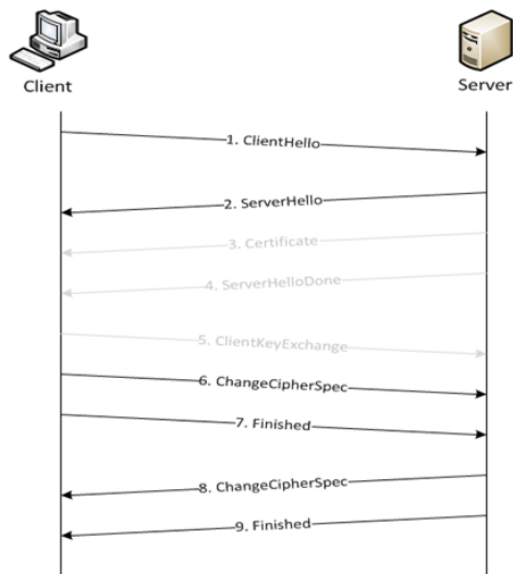
Figure 112 Resumed SSL Handshake
