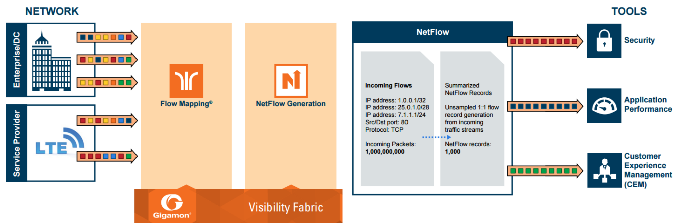
Figure 67 NetFlow Generation Gigamon Solution
