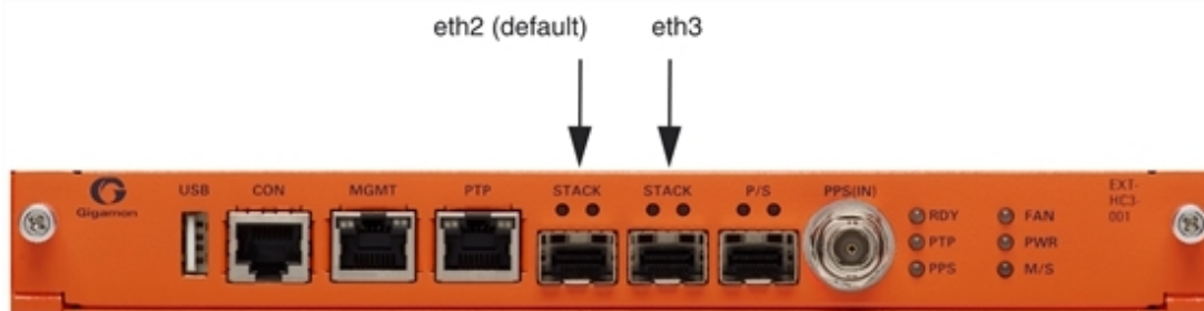
Figure 94 Stack Port Location on GigaVUE-HC3 Front
