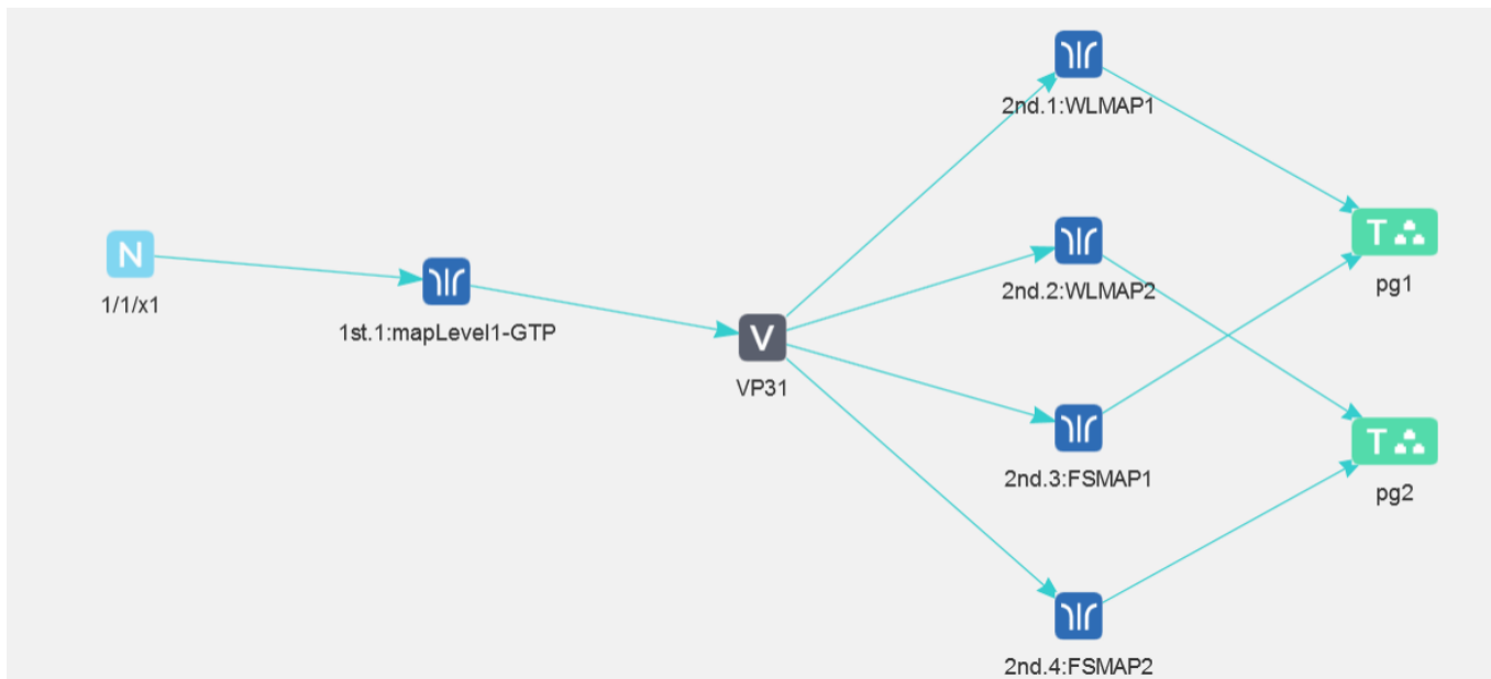
Figure 10 GTP Overlap Mode Example 1
