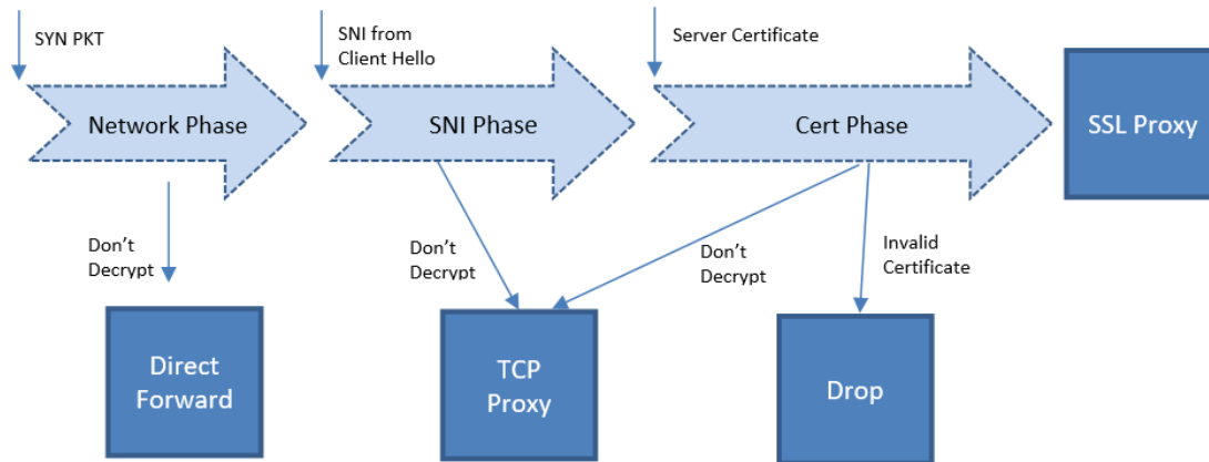
Figure 84 Policy Validation Flow
