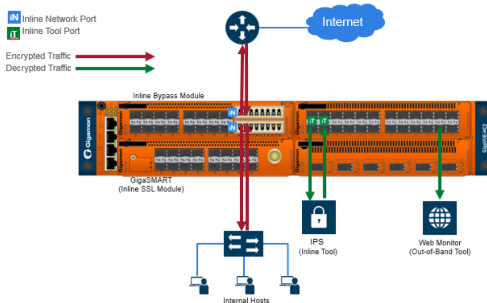
Figure 91 GigaVUE Modules: GigaSMART and Inline Bypass
