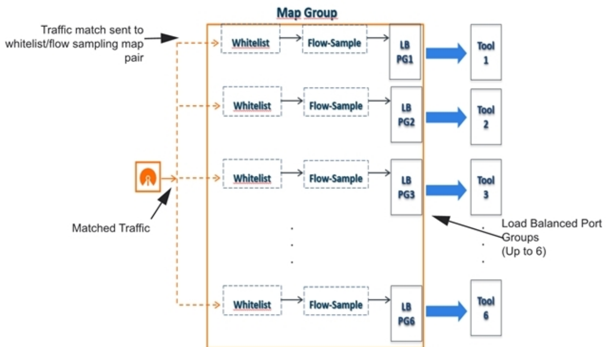
Figure 9 GTP Overlap Flow Sampling Map Groups
